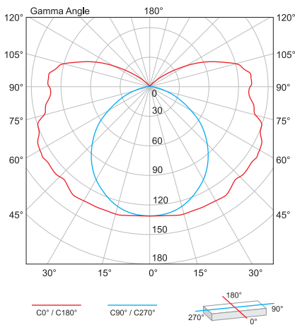
BELLA / 1X18W
