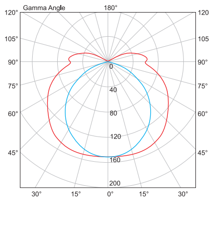
BELLA / 2X36W
